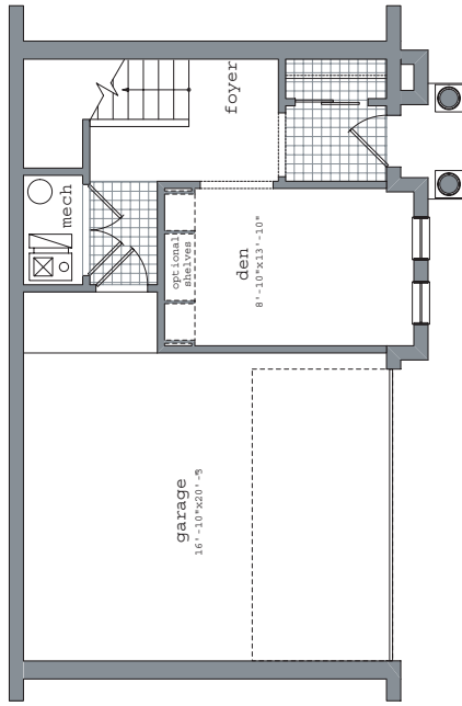
FIRST FLOOR PLAN 350 square feet
