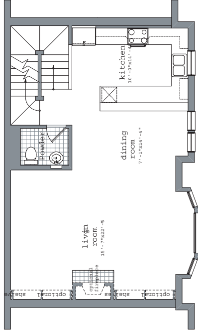
SECOND FLOOR PLAN 775 square feet
